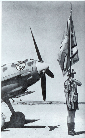
THIS PAGE: Bf 109 E-7 Trop, 'Yellow 4' of 3./JG 27 in the late Summer of 1941. Later, following the Allied advance into Cyrenaica which began on 9 December 1941, the remains of this aircraft, without wings or engine, were discovered on an abandoned airfield by British troops.
